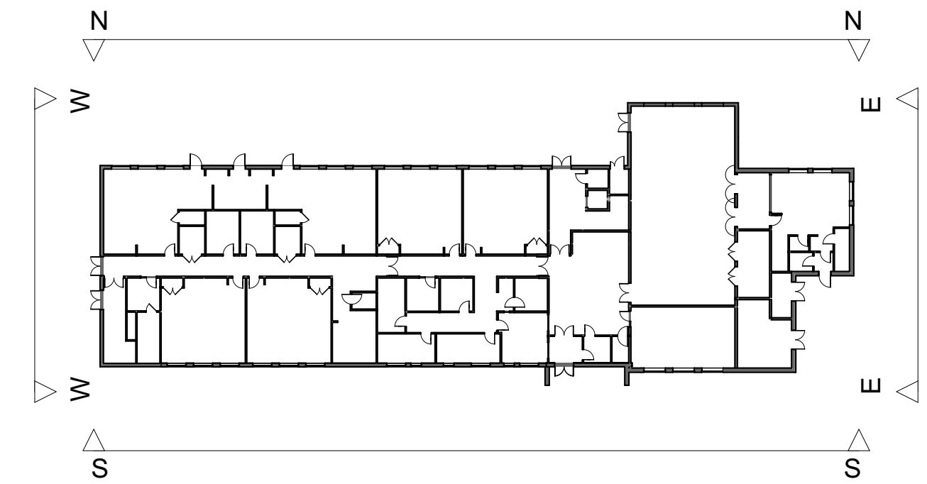
Key Plan - 1:500
