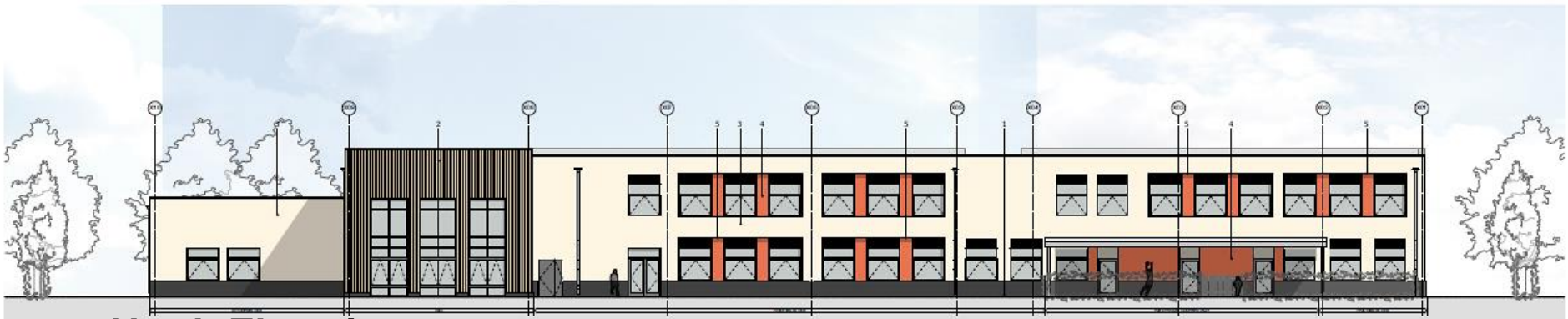
North Elevation
